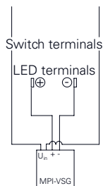
Connection Diagram for 4-Wire Systems
