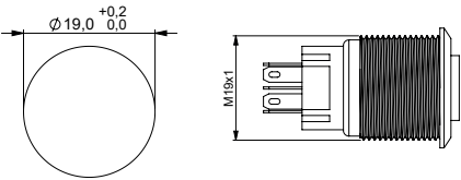
Mounting Dimensions
